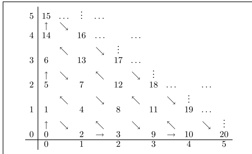
A Counted Union of Counted Sets is Counted
